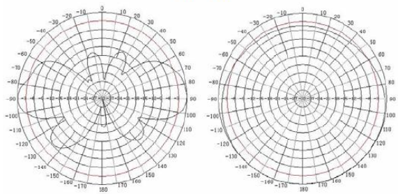
E-Plane Pattern
