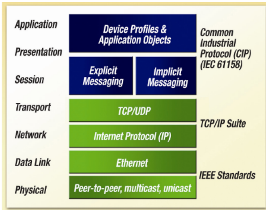
Figure 1: EtherNet/IP Protocol Stack
