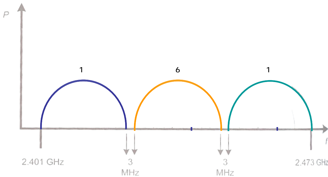
Figure 5. Non-overlapping 802.11bg Channels (1, 6 & 11)
