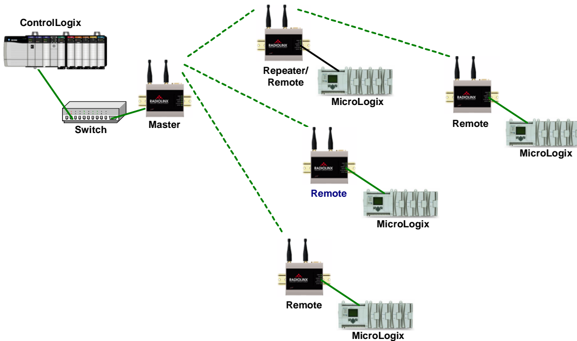
Figure 9. Wireless TCP/IP System using Explicit Messaging for Data Exchange
