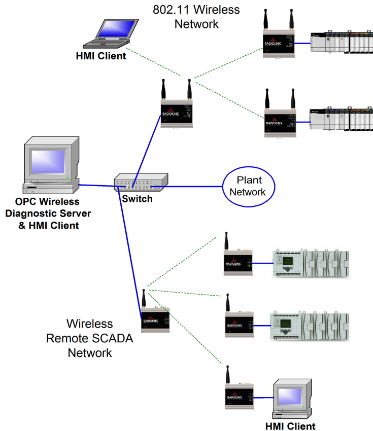
Diagram 1. The Wireless OPC Server collects diagnostic data from two separate RF networks. Any HMI client on the logical network has access to the diagnostic information.
