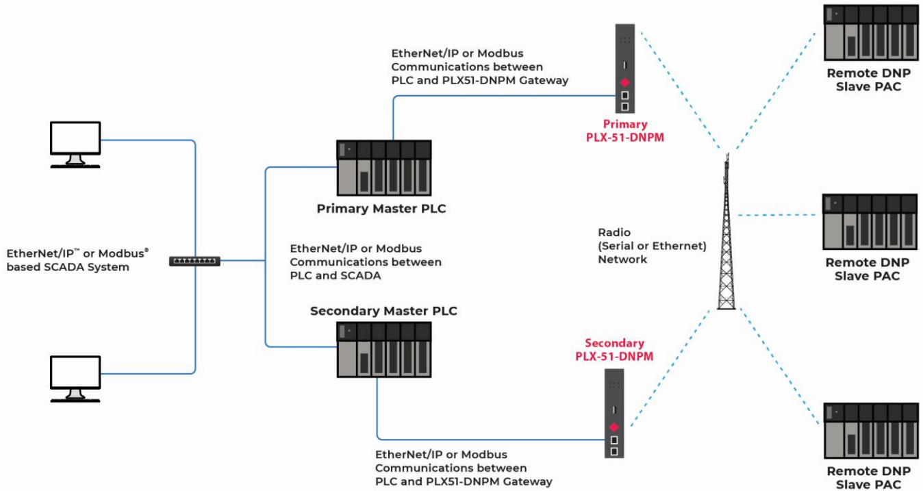
Figure 1 – PLX51-DNPM in Master mode
