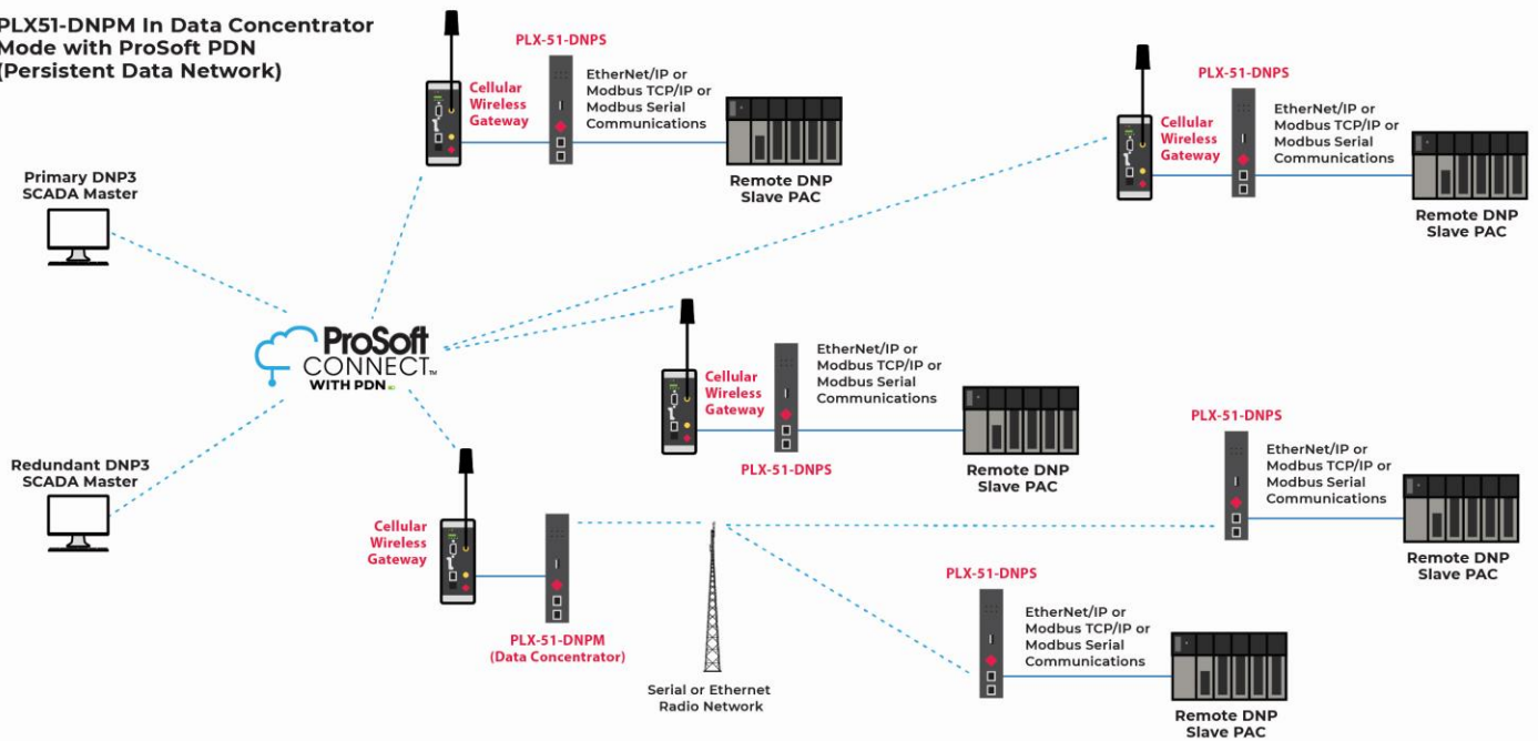
Figure 2 – PLX51-DNPM in Data Concentrator Mode
