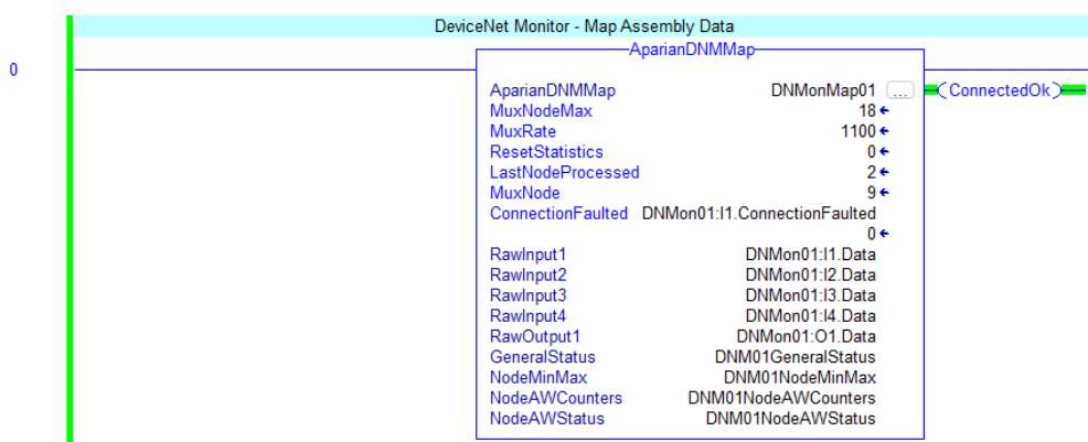
Figure 5.1 – DeviceNet Monitor AOI
